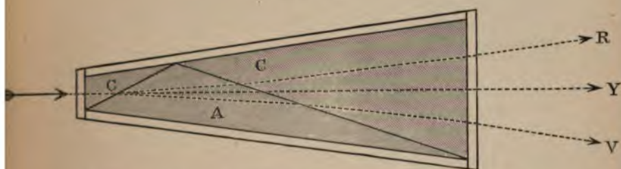
Direct-vision prism. A, wide-angled prism of Jena glass; C, cinnamic ether.
